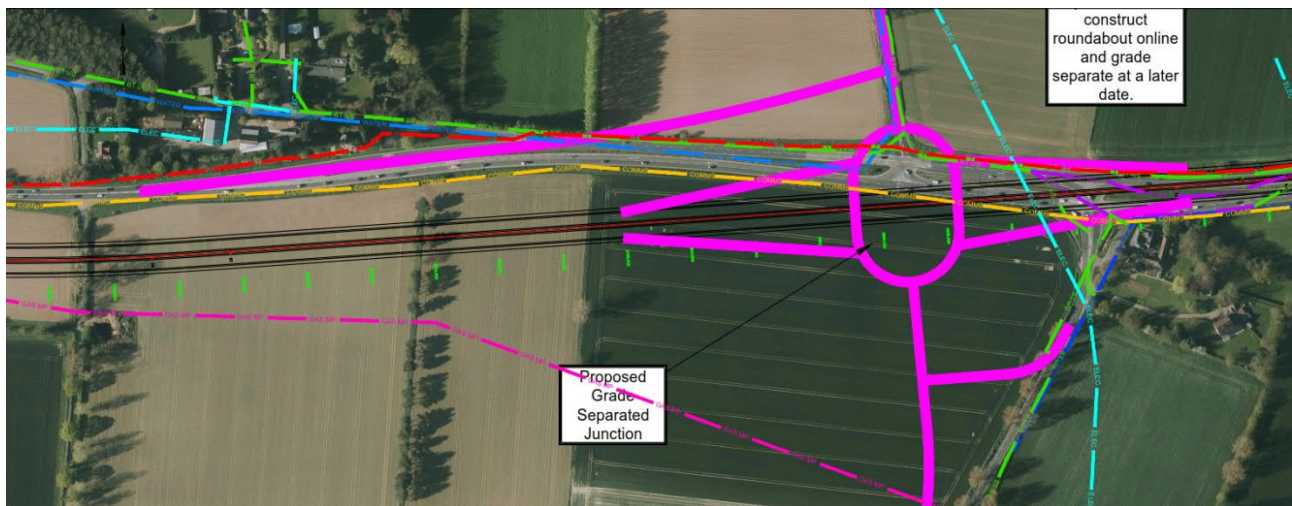
Figure 0-12: B1140 junction arrangement, Option C
