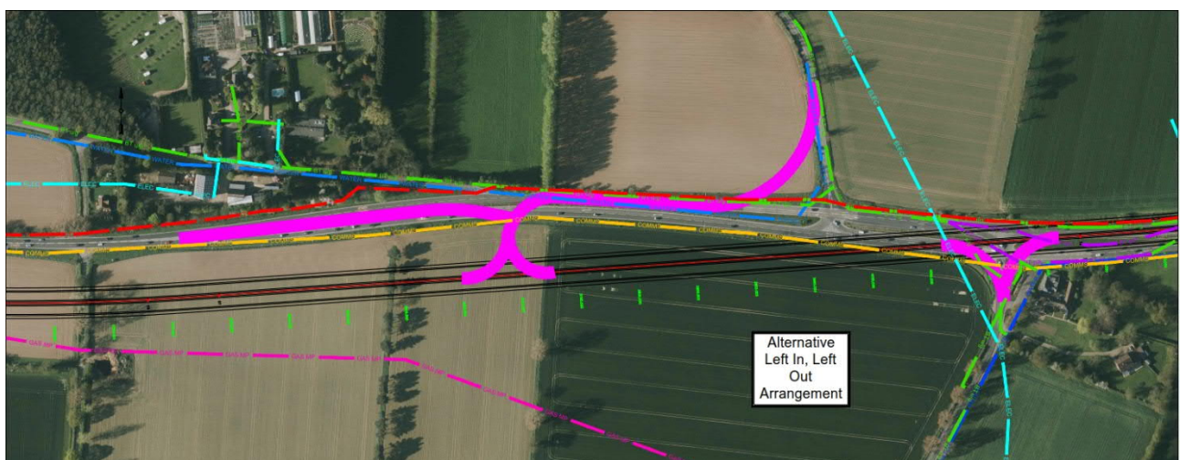
Figure 0-13: B1140 junction arrangement, Option D
