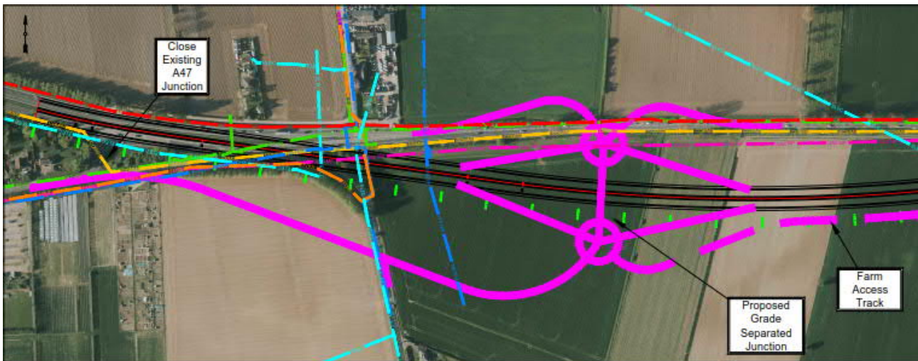
Figure 0-6: Yarmouth Road junction arrangement, Option B
